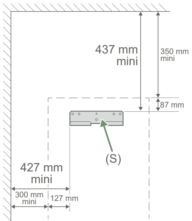
fig. 20 - Wandmontage
