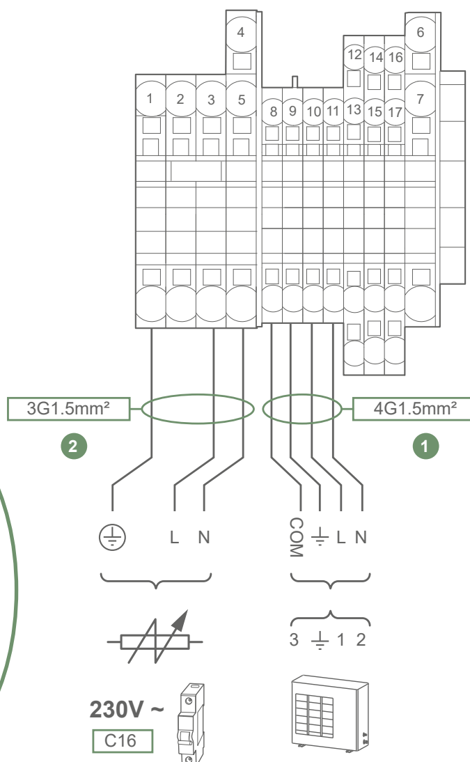
fig. 12 - Raccordements Alimentations
